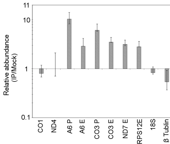
Supplementary Fig. 1. Enrichment of pre-edited and edited mRNAs pulled down with GAP1/2 immunoprecipitations in the MRB8620 RNAi knockdowns as compared to the mock pulldowns performed with unconjugated Protein G Dynabeads. Relative abundance is calculated by \Delta\text{CtIP}/\Delta\text{CtMock} as in Madina et al. (2014). Labelled as in Fig. 5B.
