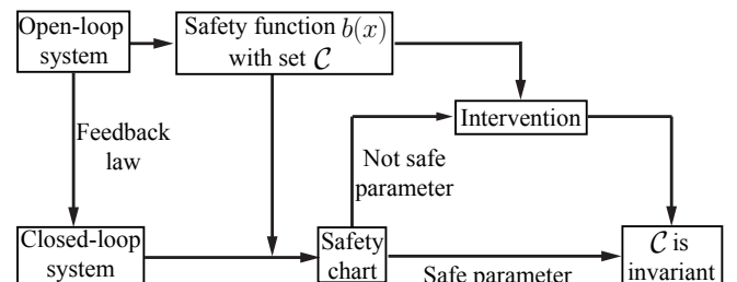
Fig. 3: Ensuring safety of a given feedback law.
