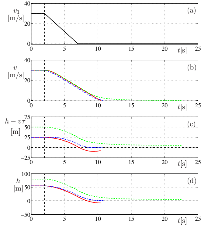
Fig. 5: Simulation results when the predecessor applies heavy braking as shown by the speed profile in panel (a). The dashed green and the solid red curves in panels (b,c,d) correspond to the safe and unsafe parameter combinations marked by a green and red crosses in Fig. 4. The blue profiles also correspond to the unsafe combination but with the intervening controller (36).
