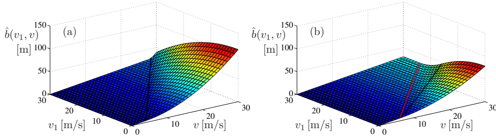
Fig. 2: Surface of \hat{b}(v_1, v) defining the safe distance for minimum time headway \tau = 1 [s]. (a) The case given by (13) for \underline{a} = 4 [m/s 2 ] and \underline{a}_1 = 6 [m/s 2 ] with the black line indicating the switch (14). (b) The case given by (15) for \underline{a} = 6 [m/s 2 ] and \underline{a}_1 = 4 [m/s 2 ] with the black and red lines indicating the switches (16).
