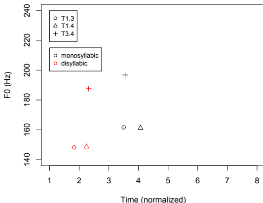
F0 Minima by Word Size, Simple Rising tones
