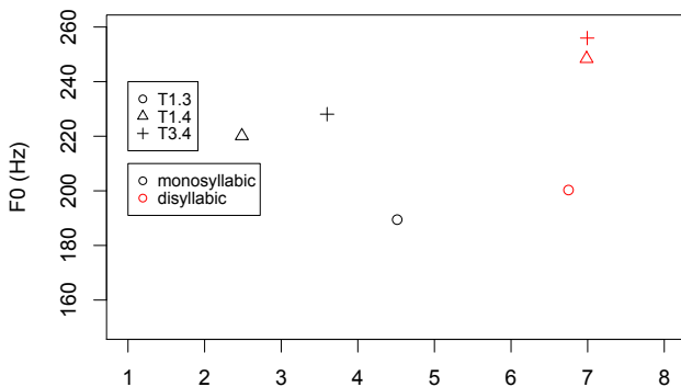
F0 Maxima by Word Size, Simple Rising tones
