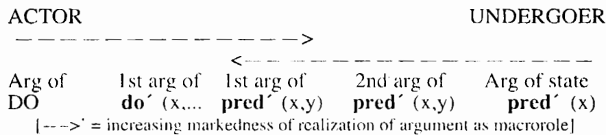
Figure 5: The Actor–Undergoer Hierarchy 1
