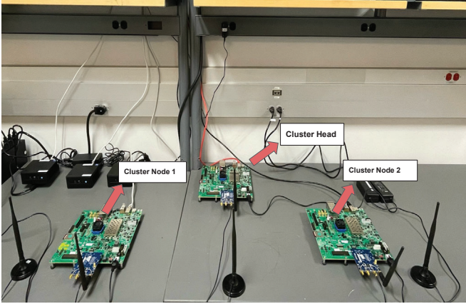
Fig. 2: Testbed Setup
