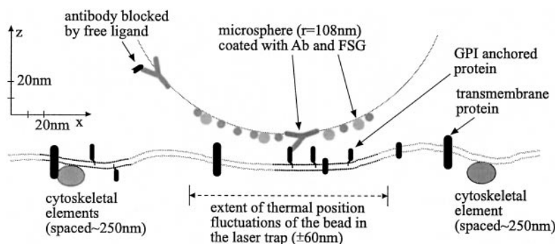
Figure 1. Scaled model of the experimental situation: a sphere ( r = 108 nm) bound via an adsorbed antibody to a GPI-anchored protein that is part of a raft domain. The lipid bilayer is symbolized by the double row of gray dots with black sections symbolizing raft domains. The extent of the thermal position fluctuations observed in the experiments ( \pm 60 nm) is marked. It is much smaller than the smallest estimates of the spacing of immobile cytoskeleton-anchored obstacles to free diffusion of 300–500 nm (Sako and Kusumi, 1995). The cytoskeletal elements drawn here are 250 nm apart.
