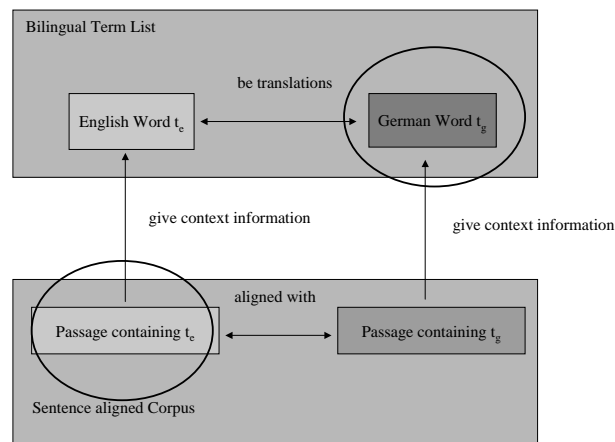
Figure 5: Constructing cross-language KWIC using a sentence-aligned parallel corpus.
