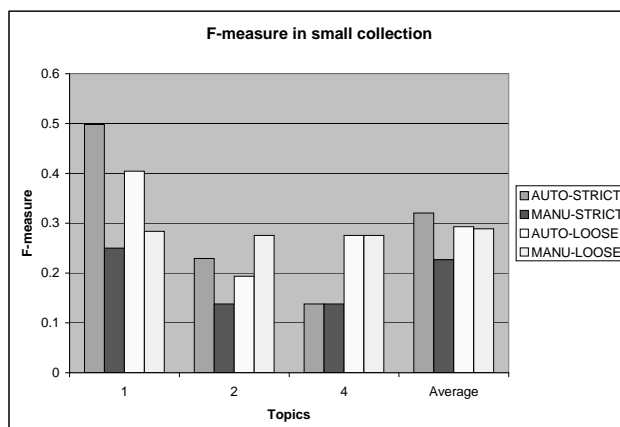
Figure 7: F_{\alpha} = 0.8 , small collection group, by condition.
