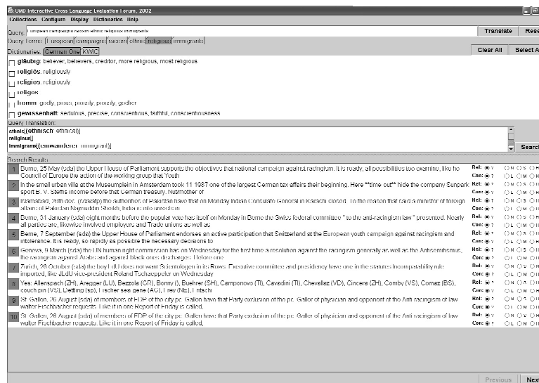
Figure 3: User interface, manual condition.
