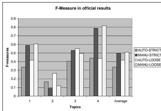
Figure 6: F_{\alpha} = 0.8 , large collection, by condition and topic.
